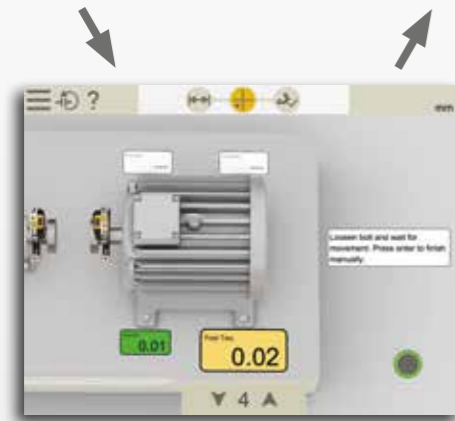
Soft Foot check
